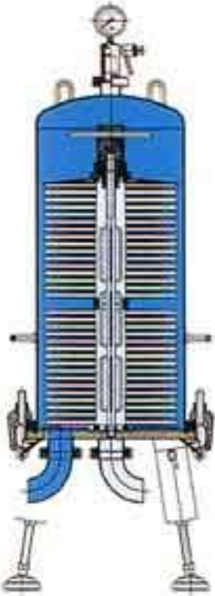
Cross sectional view with in/out lets
